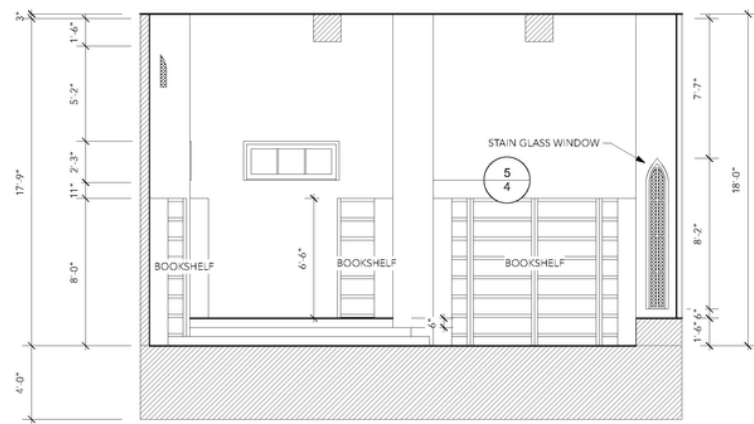
A INT. Shivers' Study - Elevation Scale: 1/4" = 1'-0"
