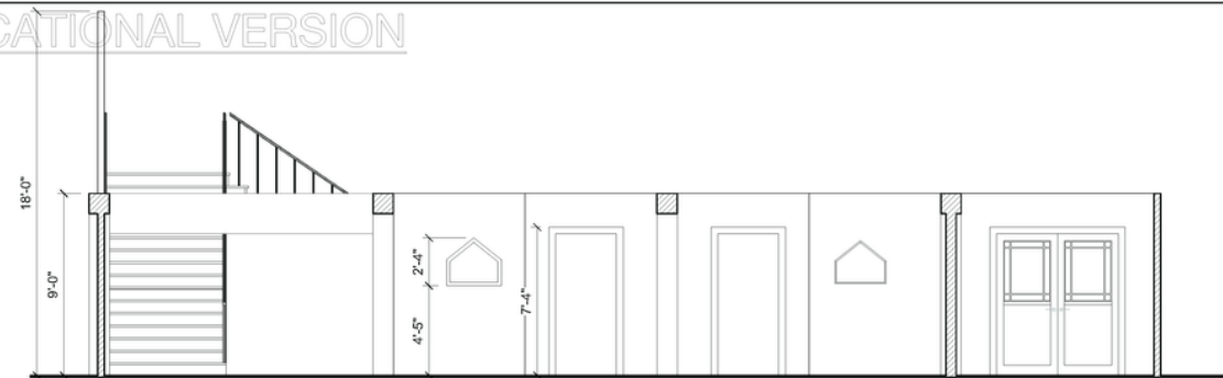
2 Section Elevation - Station Set Scale: 1/4" = 1'-0"
