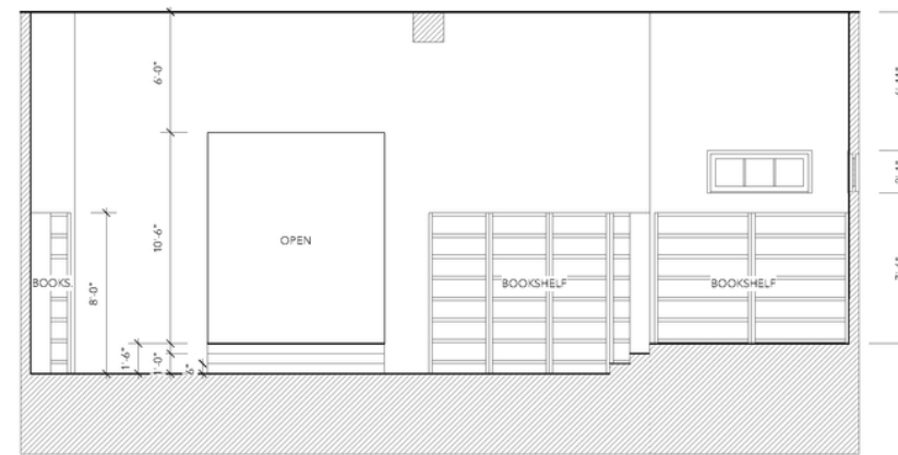
D INT. Shivers' Study - Elevation Scale: 1/4" = 1'-0"
