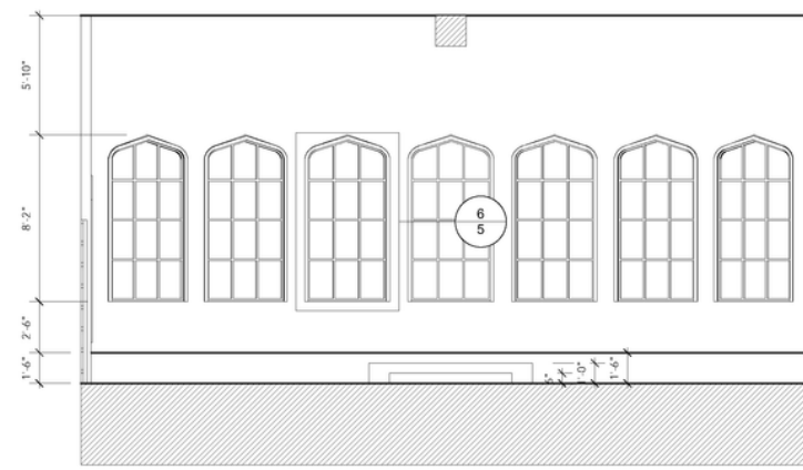
B INT. Shivers' Study - Elevation Scale: 1/4" = 1'-0"
