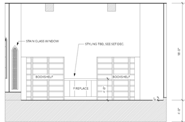
C INT. Shivers' Study - Elevation Scale: 1/4" = 1'-0"
