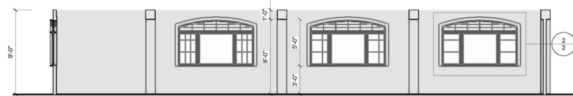
1 Section Elevation - Station Set Scale: 1/4" = 1'-0"
