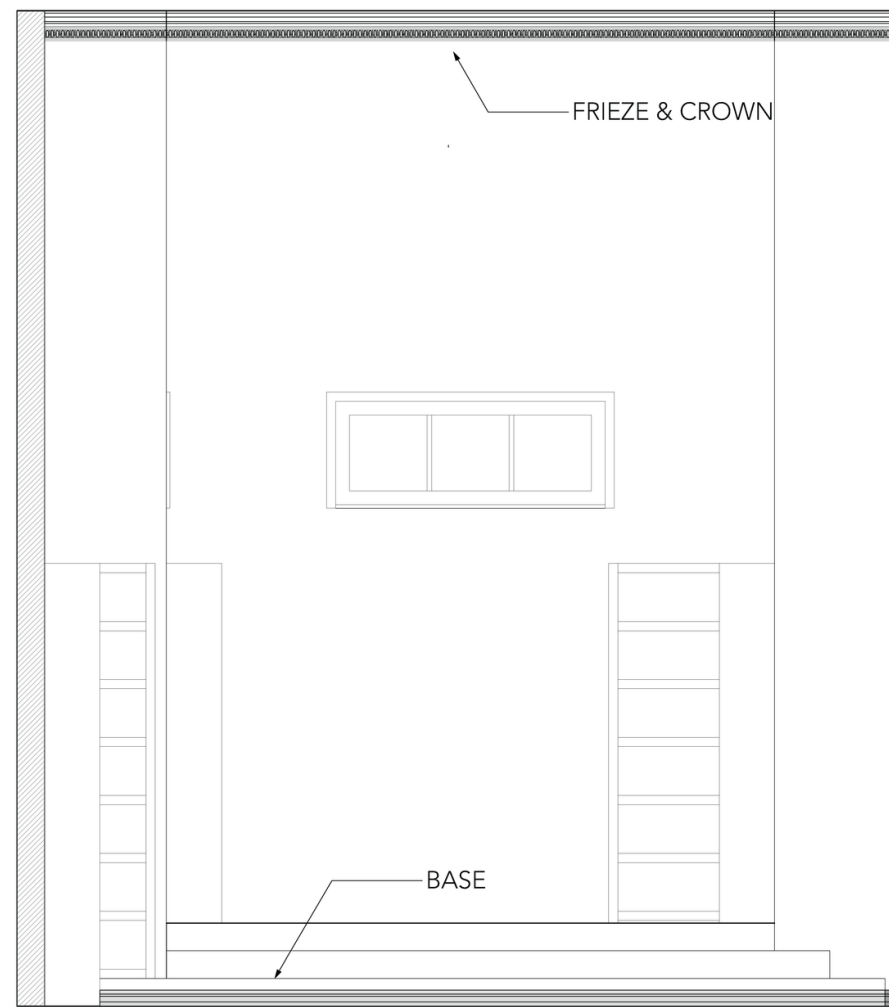
5 INT. Shivers - Wall Detail Scale: 3/4" = 1'-0"
