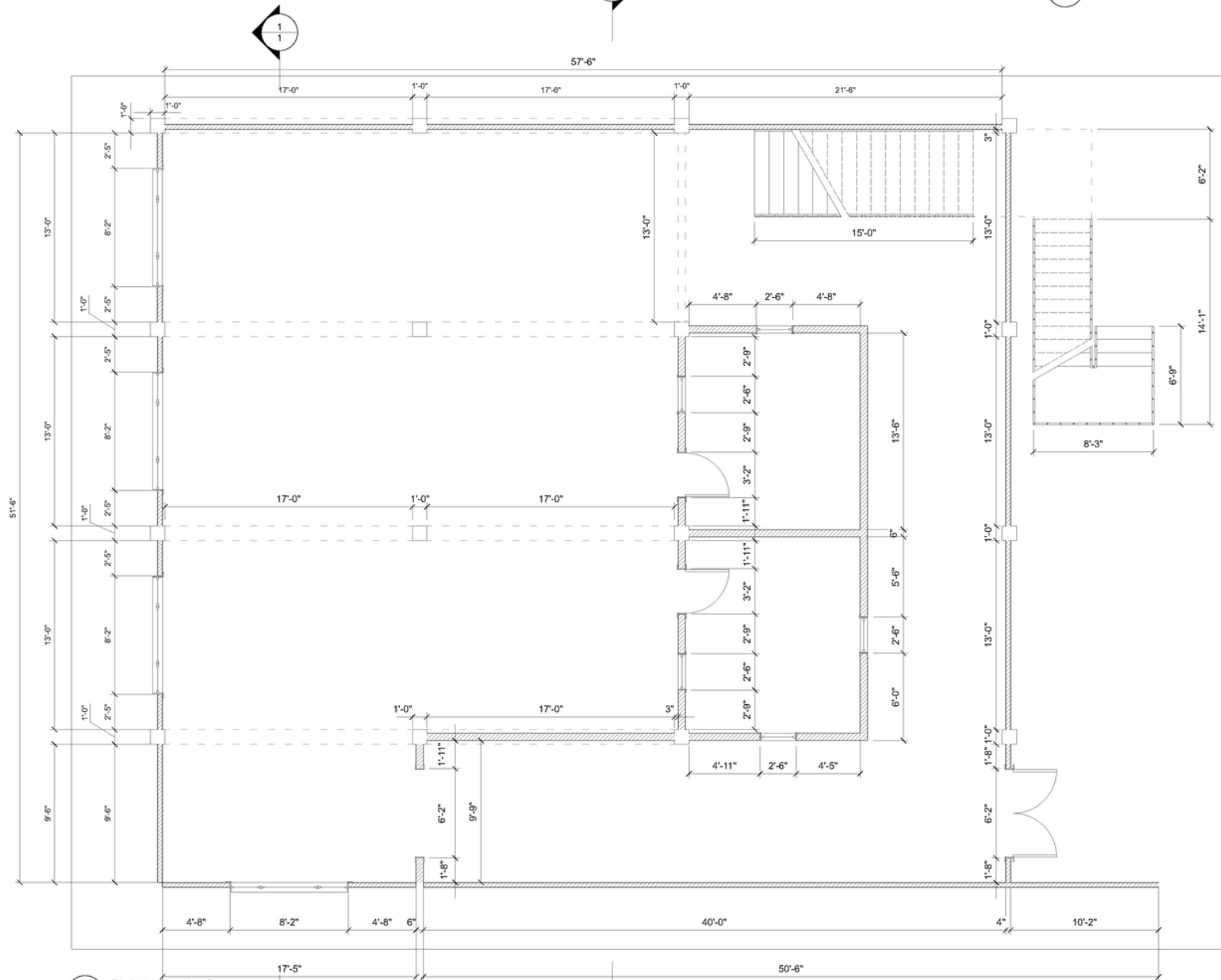
A PLAN - Station Set Scale: 1/4" = 1'-0"
